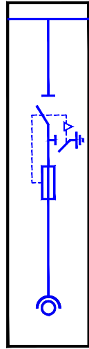
MİMİK DİYAGRAM
